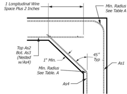
FIG. 11 Alternate Detail
