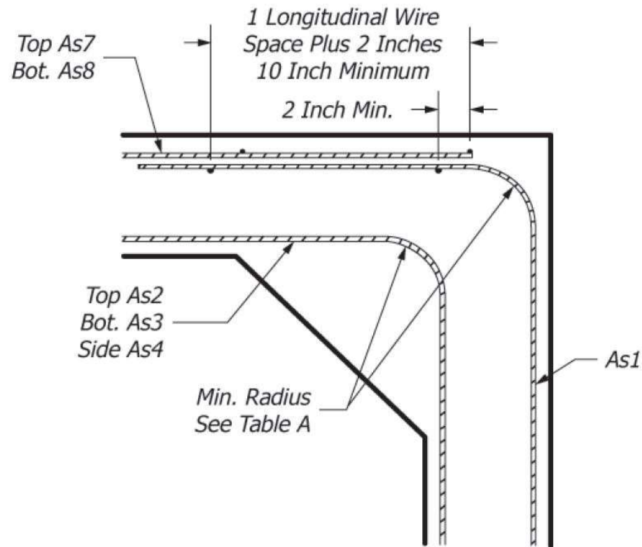
FIG. 6 Detail Option
