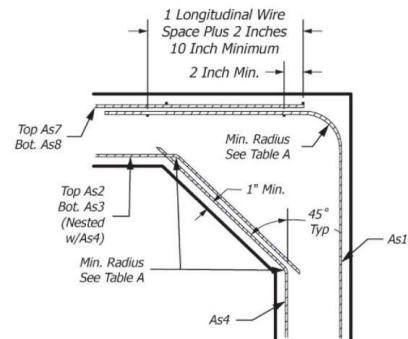
FIG. 14 Alternate Detail
