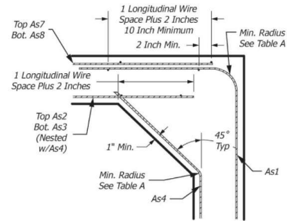
FIG. 12 Alternate Detail
