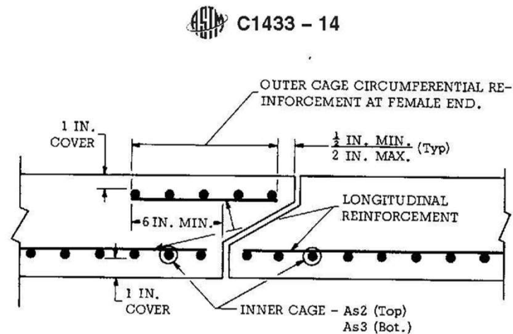
FIG. 2 Section A-A Top and Bottom Slab Joint Reinforcement
