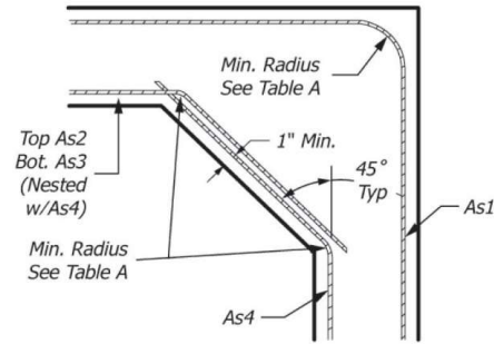
FIG. 13 Alternate Detail
