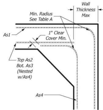
FIG. 9 Alternate Detail
