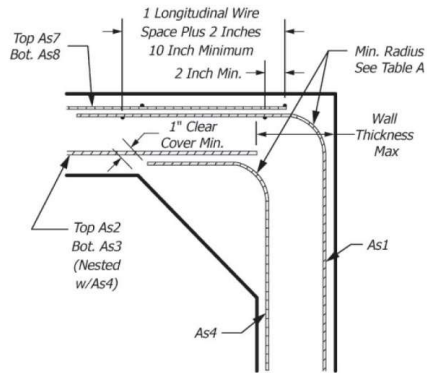
FIG. 10 Alternate Detail
