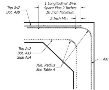
FIG. 6 Detail Option
