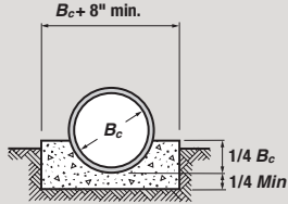
CONCRETE CRADLE CLASS A
