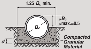
GRANULAR FOUNDATION CLASS B
