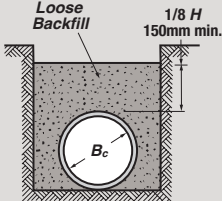
FLAT SUBGRADE CLASS D B_f = 1.1
