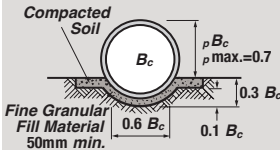
SHAPED SUBGRADE WITH GRANULAR FOUNDATION
