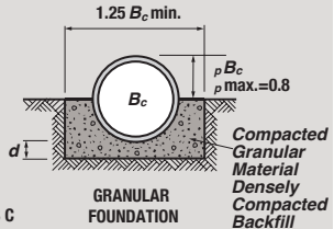
GRANULAR FOUNDATION
