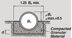
GRANULAR FOUNDATION
